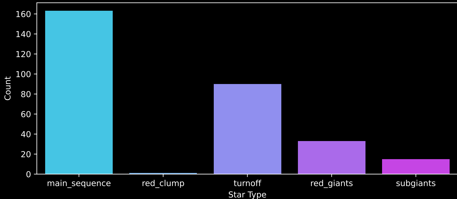
GALAH DR4 Field: [205] Count plot of Star Type
