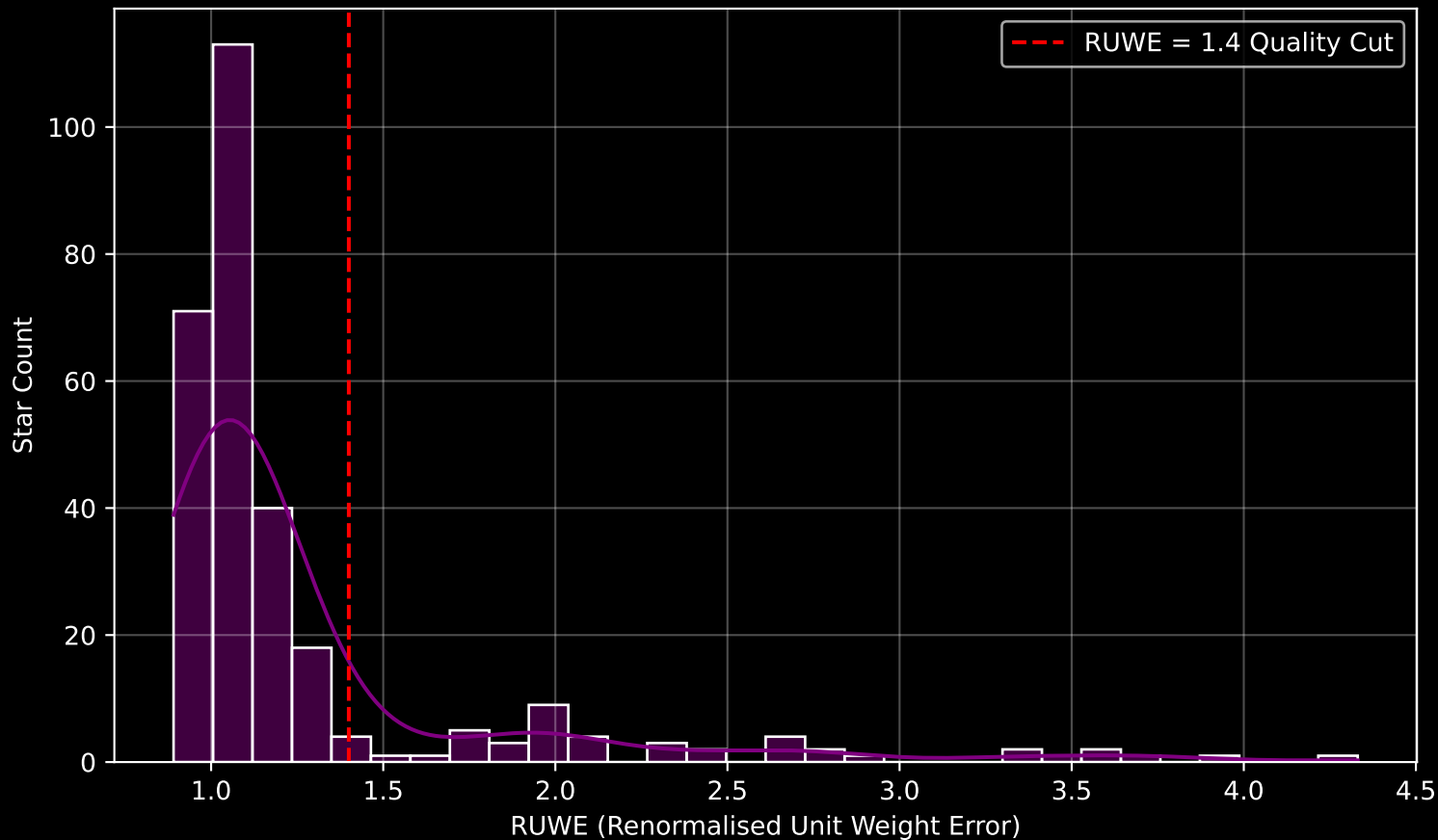
GALAH DR4 Field [205] RUWE Distribution (n= 289)
