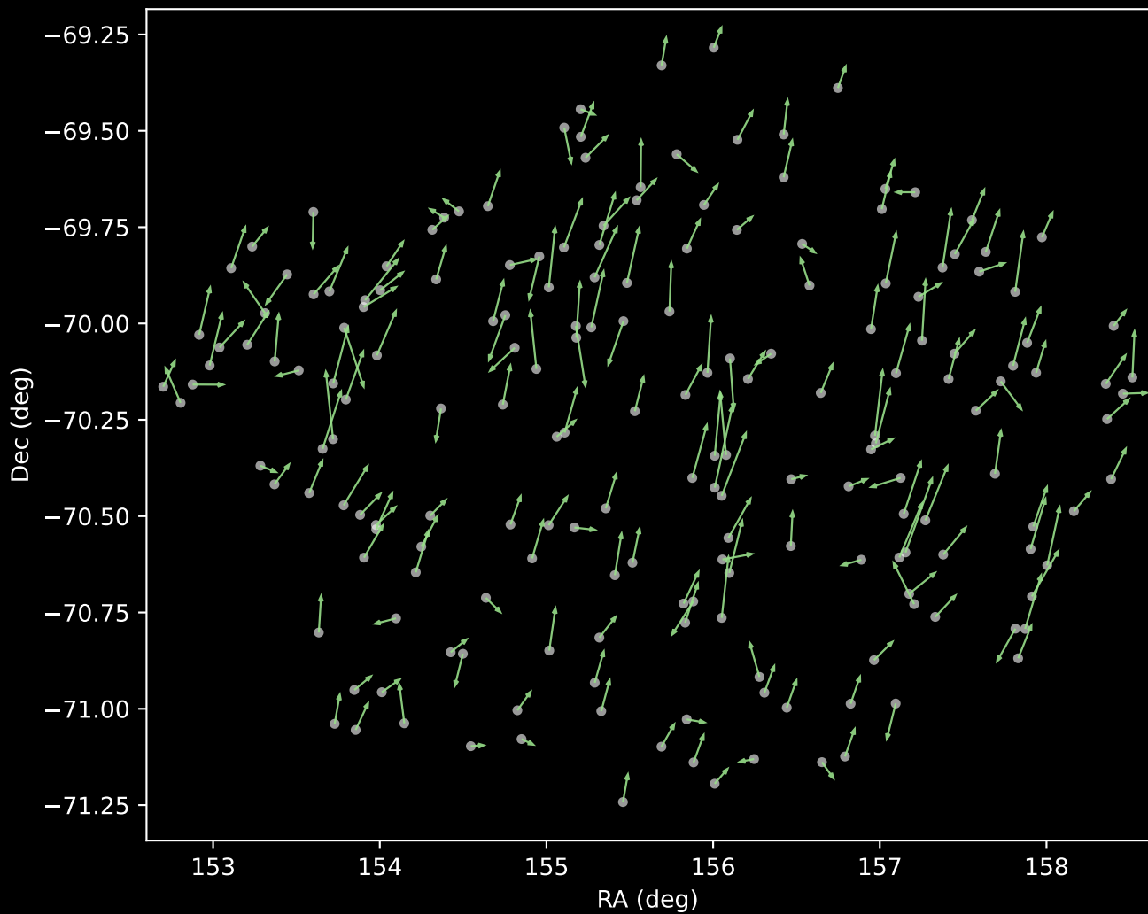
GALAH DR4 Cluster 5 Proper Motion Vectors (n=191)
